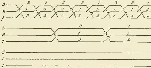
Fig. 23. Transposition Diagram of Three Parallel Three-Phase Lines to Reduce Mutual-Inductance
